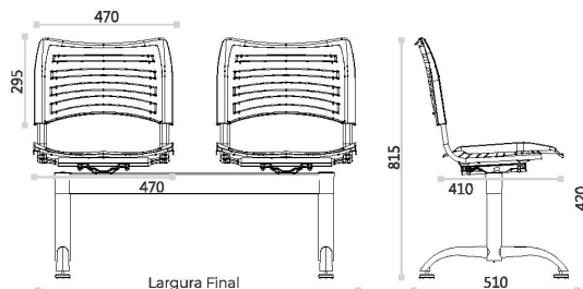
FIT LONGARINA CELTA
