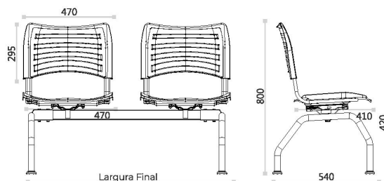
FIT LONGARINA ARKO
